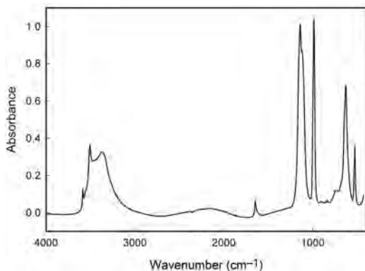
FIG. 2. The IR spectrum of steverustite.
