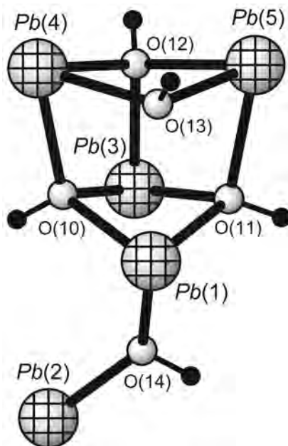
FIG. 5. The strongly bonded \text{Pb}_5(\text{OH})_5 unit in steverustite. Legend as in Fig. 3.
