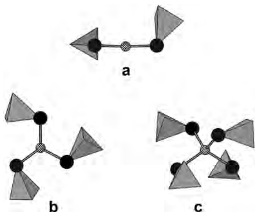
FIG. 9. Known [(\text{S}_2\text{O}_3)_n\text{-X}] groups in crystal structures: (a) the linear [\text{Au}(\text{S}_2\text{O}_3)_2]^{3-} group in \text{Na}_3\text{Au}(\text{S}_2\text{O}_3)_2(\text{H}_2\text{O})_2 , (b) the triangular [\text{Cu}(\text{S}_2\text{O}_3)_3]^{5-} group in steverustite, and (c) the tetrahedral [\text{X}(\text{S}_2\text{O}_3)_4]^{7-} group in (\text{NH}_4)_9\text{Br}_2[\text{Ag}(\text{S}_2\text{O}_3)_4] and \text{Na}_4\text{Ni}(\text{NH}_3)_4[\text{Ag}(\text{S}_2\text{O}_3)_2]_2(\text{NH}_3) with [\text{X} = \text{Ag}] , and \text{Na}_4\text{Cu}(\text{NH}_3)_4[\text{Cu}(\text{S}_2\text{O}_3)_2]_2(\text{NH}_3) with [\text{X} = \text{Cu}] . Legend as in Fig. 4, with the \text{X} cation diagonally cross-hatched.
