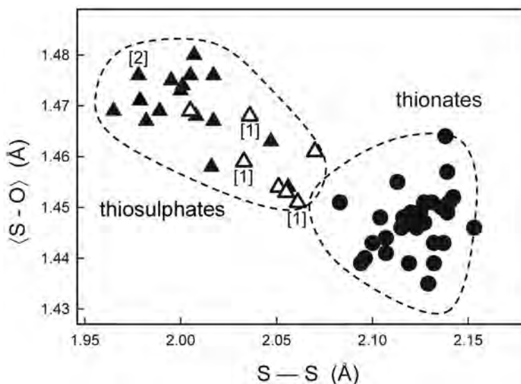
FIG. 10. The \langle \text{S}^{6+}\text{–O} \rangle distance as a function of S–S distance for the compounds listed in Appendix A (available for download from www.minersoc.org/pages/e_journals/dep_mat_mm.html ); black circles: thionate groups; black triangles: thiosulphate groups in which the \text{S}^{2-} atom bonds to cation ( \text{X} ) – (O,N) (cf. Fig. 8c); open triangles: thiosulphate groups in which the cation ( \text{X} ) bonds only to \text{S}^{2-} atoms (cf. Fig. 8d). Data belonging to steverustite and sidpietersite are labelled [1] and [2], respectively.
