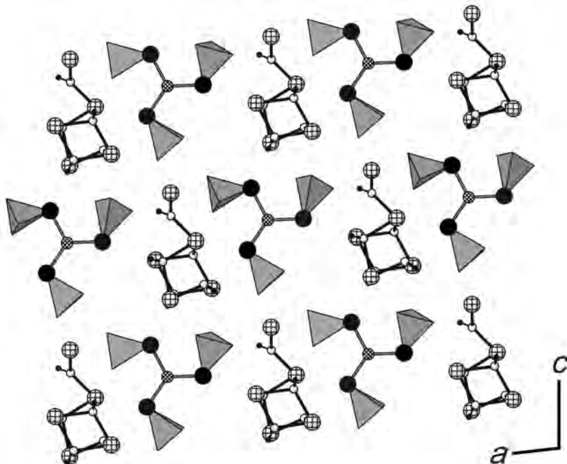
FIG. 6. The (010) layer of alternating \text{Pb}_5(\text{OH})_5 and \text{Cu}(\text{S}_2\text{O}_3)_3 groups in steverustite. Legend as in Figs 3 and 4. Note that the longer Pb— \phi bonds are not drawn.
