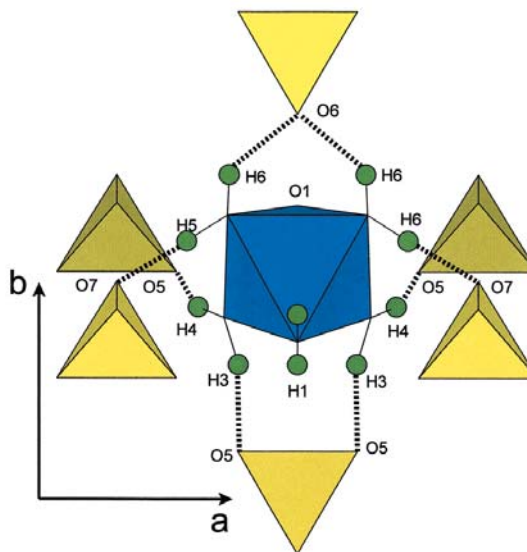
FIG. 1. Coordination polyhedra and hydrogen bonding in orthominasragrite; (VΦ 6 ) octahedron: blue; (SO 4 ) tetrahedron: yellow; H atoms: green circles; hydrogen bonds: broken lines. The variation in yellow shading denotes height relative to the plane of the diagram.
