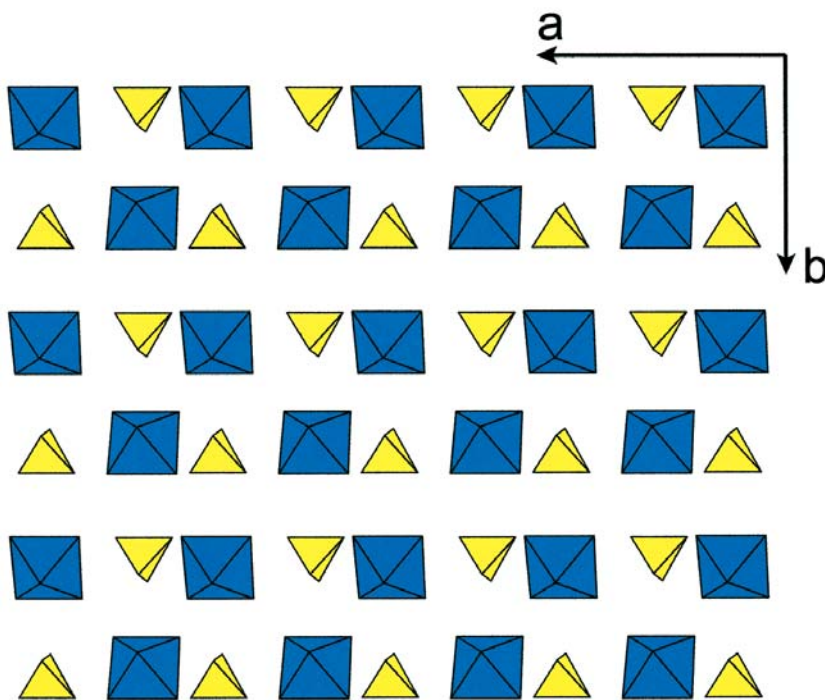
FIG. 2. The (VΦ 6 ) and (SO 4 ) polyhedra in orthominasragrite viewed down the c axis; legend as in Figure 1.
