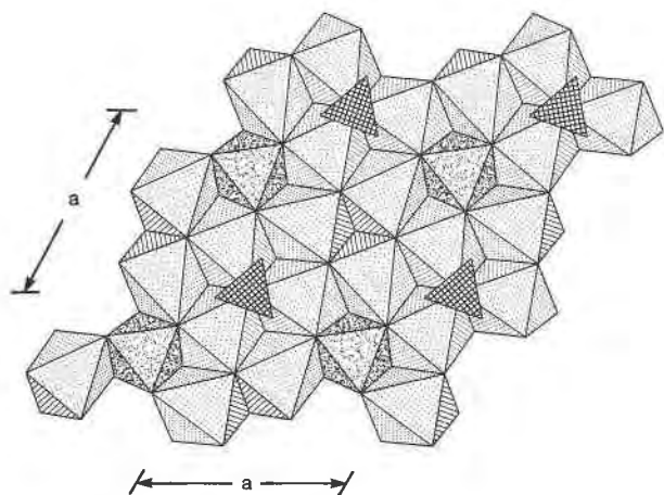
Fig. 1. The \text{Cu}_6\text{Al}(\text{SO}_4)(\text{OH})_{12}\text{Cl} sheet in spangolite viewed along [001]; \text{Cu}_6\phi_6 octahedra are shaded with dots in a regular pattern, \text{Al}_6\phi_6 octahedra are shaded in an irregular pattern, \text{SO}_4 tetrahedra are cross-hatched.
