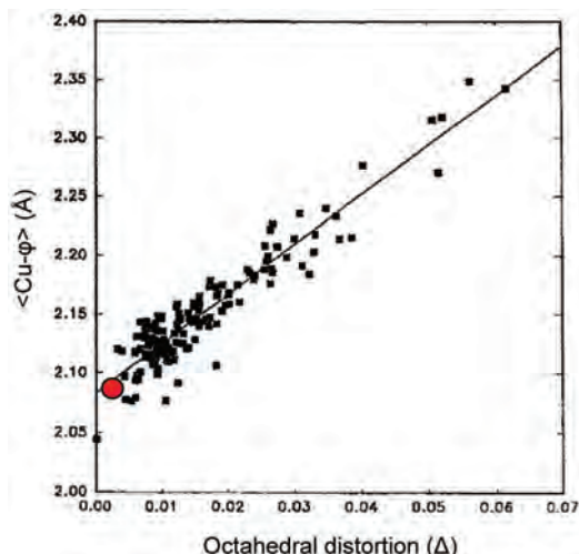
FIG. 3. \langle ^{[6]}\text{Cu}^{2+}-\text{O} \rangle distance as a function of the deviation, \Delta , of the Cu–O bond lengths from their mean value, where \Delta = \Sigma[(l - l_0)/l_0]^2/6 , l is the individual bond length and l_0 is the mean bond length; the data for chalcoalumite is shown as a red circle. Modified from Burns and Hawthorne (1996).
