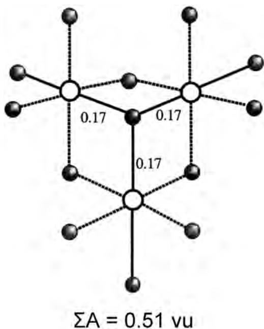
FIG. 5. Typical local bond-valence arrangement for an (\text{SO}_4)^{2-} or (\text{H}_2\text{O})^0 group to link to a [\text{Cu}^{2+}\phi_2]_N sheet; \text{Cu}^{2+} cations are shown as white circles, anions are shown as highlighted dark circles, bond valences are shown around the central anion, apical (elongated) bonds are shown as full lines, equatorial bonds are shown as dotted lines. Note that three apical (long) \text{Cu}^{2+}-\phi bonds must link to the same anion to provide an incident bond valence, A, appropriate for \phi = (\text{SO}_4)^{2-} or (\text{H}_2\text{O})^0 . From Hawthorne and Schindler (2000).
