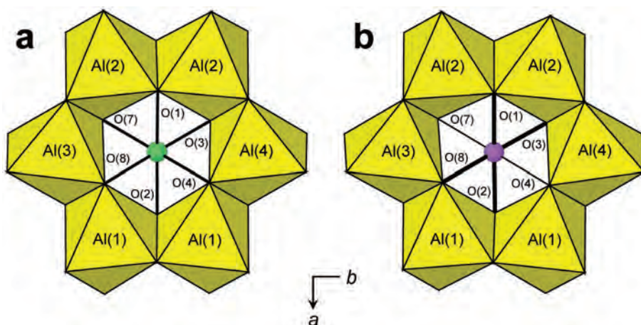
FIG. 4. Comparison of the atomic arrangements around the Ni and Cu sites in (a) nickelalumite, and (b) chalcoalumite; legend as in Fig. 2, the thickness of the Ni–O and Cu–O bonds are proportional to their bond valence.
