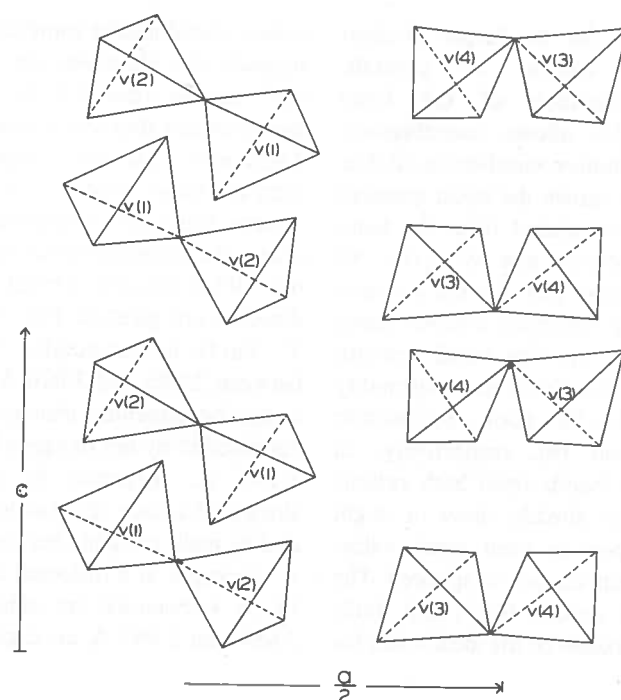
FIG. 2. An ac projection of the structure of Ba_2V_2O_7 , showing the configurations of the divanadate groups. The typical dichromate-type sheets are seen here edge on.
