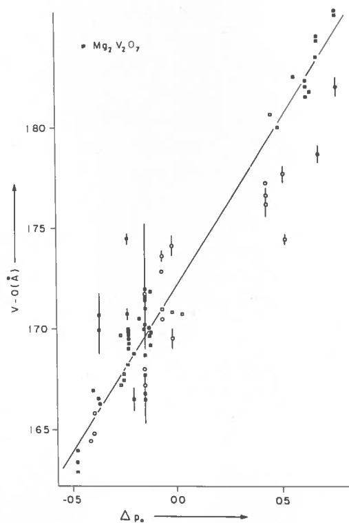
FIG. 7. The variation in V-O as a function of \Delta p_0 (see text). The solid line is the relationship derived by Gopal (21) for tetrahedral V^{5+} -O bonds.
