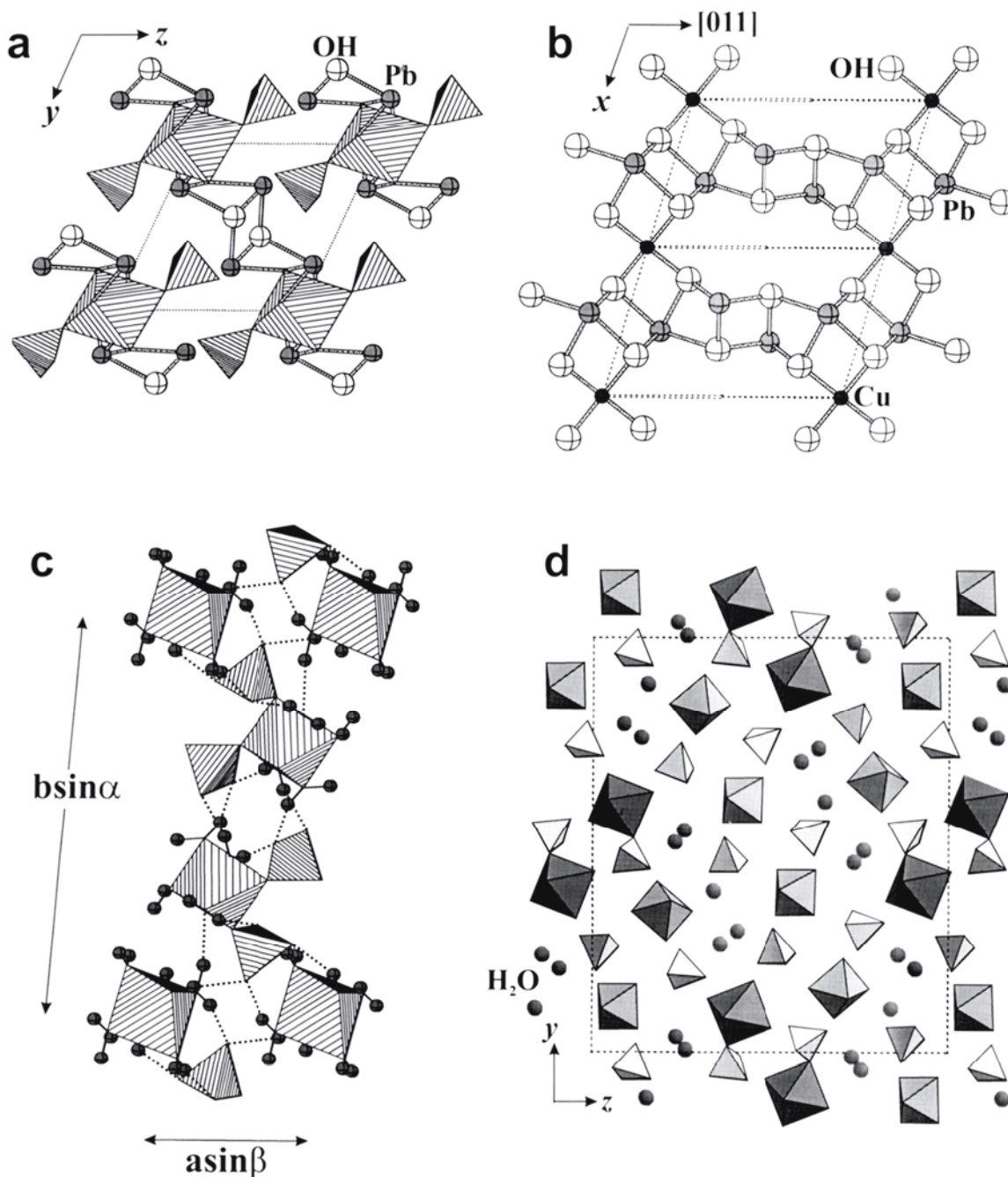
Figure 18. The structures of (a) chenite, based on [\text{Cu}(\text{OH})_4(\text{SO}_4)_2] clusters, Pb atoms, and (OH)-anions; (b) the sheet of Pb and Cu atoms and (OH)-groups in chenite; (c) r  merite; (d) apjohnite.
