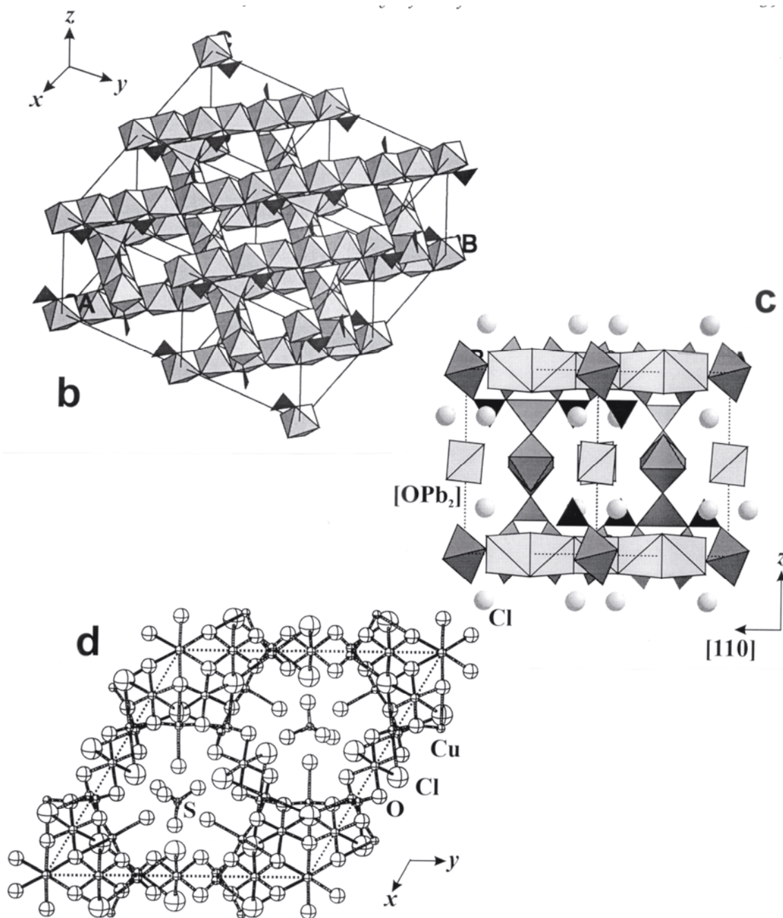
Figure 35, cont'd. (b) The trellis-like framework resulting from the intersection of the chains in (a); (c) the structure of philolite projected down [110] ; the [OPb_2] chains of edge-sharing (OPb_4) tetrahedra are shown as lightly shaded; (d) the structure of connellite projected down [001] ; the (SO_4) groups are disordered in the channels of the framework of (CuO_6) octahedra.
