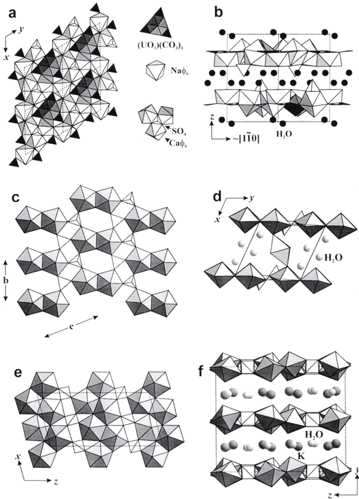
Figure 49. (a) The polyhedral sheet in schröckingerite; (b) the arrangement of sheets in the structure of schröckingerite; (c,d,e,f) the sheets of \{\text{UO}_2\}\text{O}_5 pentagonal bipyramids and (\text{SO}_4) tetrahedra and the structures of (c,d) johannite and (e,f) zippeite.
