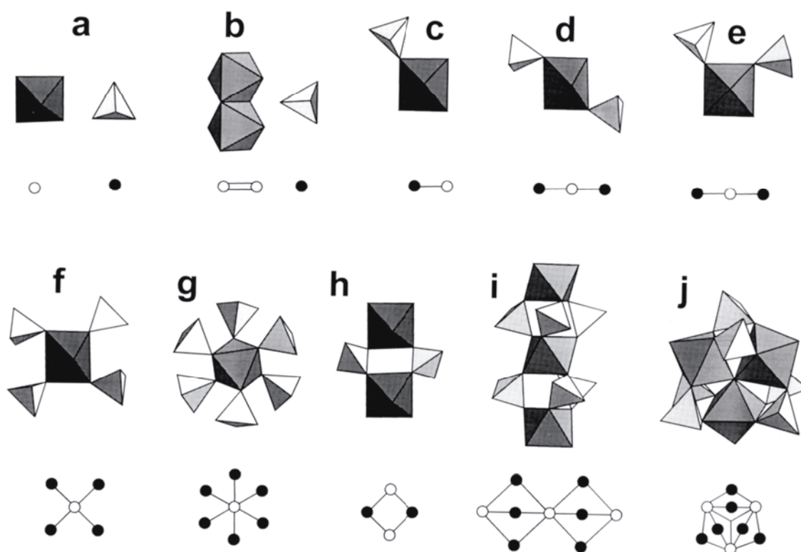
Figure 13. Finite octahedral–tetrahedral clusters in the sulfate minerals and their graphs.
