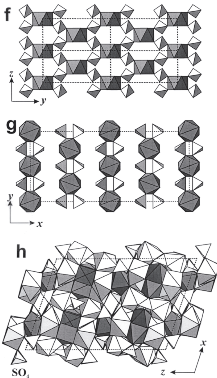
Figure 52, cont'd. (f) The sheet of (\text{ZrO}_8) polyhedra and (\text{SO}_4) tetrahedra in zircosulfate; (g) packing of the sheets in the structure of zircosulfate; (h) the structure of vonbezingite projected down [010] .
