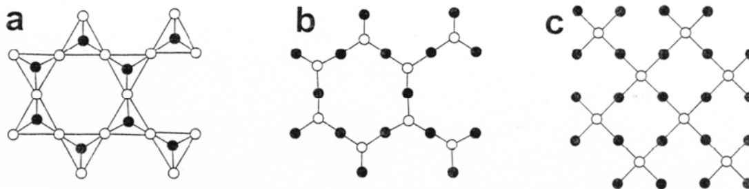
Figure 28. Graphs of the octahedral–tetrahedral sheets in the structures of sulfate minerals.
