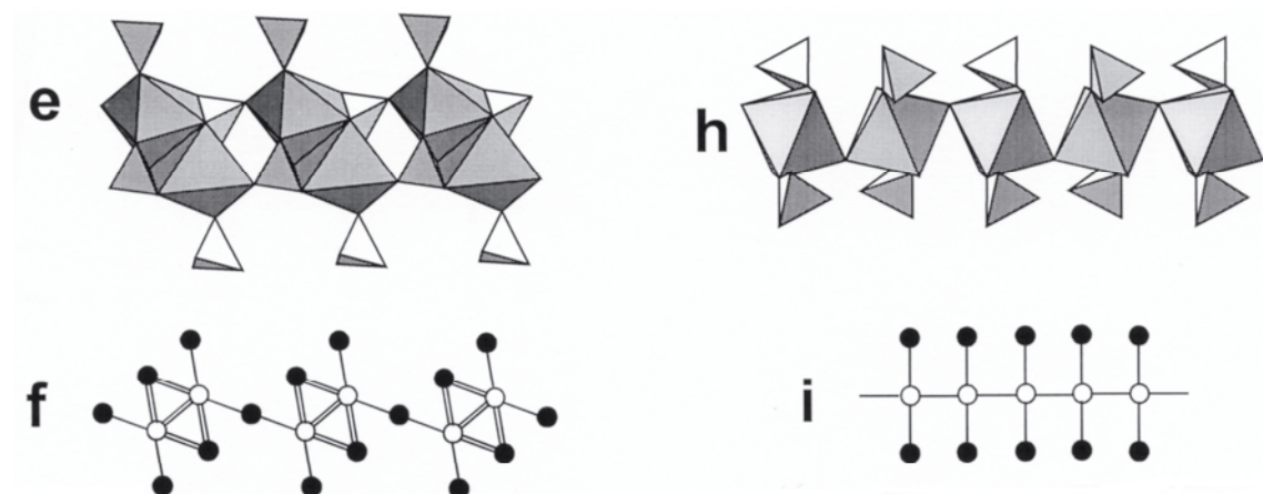
Figure 15, cont'd. The structures of sulfate minerals with isolated (SO 4 ) tetrahedra and (M \emptyset 6 ) octahedra: (e) the chain of (Na \emptyset 6 ) octahedra and (SO 4 ) tetrahedra in tamarugite; (f) the graph of the chain in tamarugite; (h) the chain of (Na \emptyset 6 ) octahedra and (SO 4 ) tetrahedra in mendozite; (i) the graph of the chain in mendozite.
