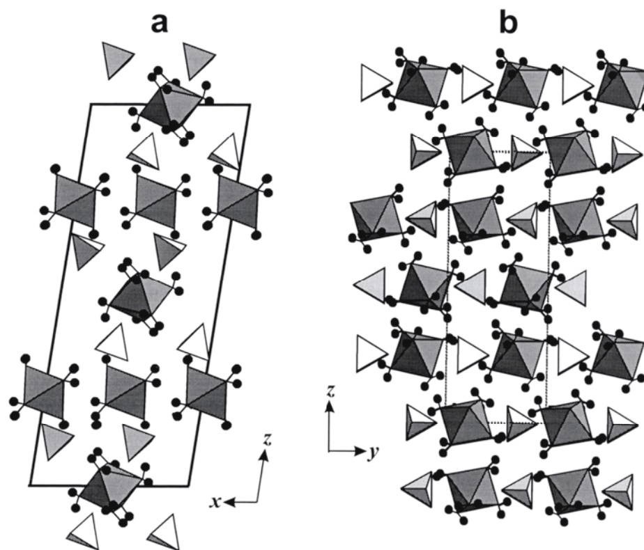
Figure 14. The structures of sulfate minerals with isolated ( \text{SO}_4 ) tetrahedra and ( \text{MO}_6 ) octahedra: (a) hexahydrite; (b) retgersite.
