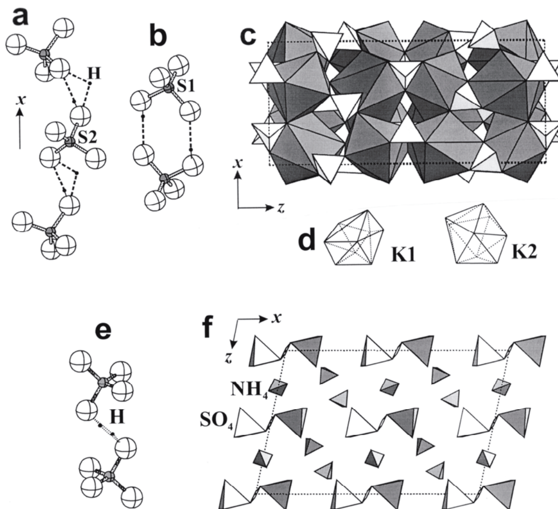
Figure 45. (a) The chain of H-bonded (\text{HSO}_4)^- groups in mercallite; (b) [(\text{HSO}_4)_2]^{2-} dimers in mercallite; (c) the structure of mercallite viewed along [010]; (d) the coordination polyhedra of K in mercallite; (e) the [(\text{SO}_4)\text{H}(\text{SO}_4)]^{3-} cluster with the disordered H atom in letovicite; (f) the structure of letovicite viewed along [010].
