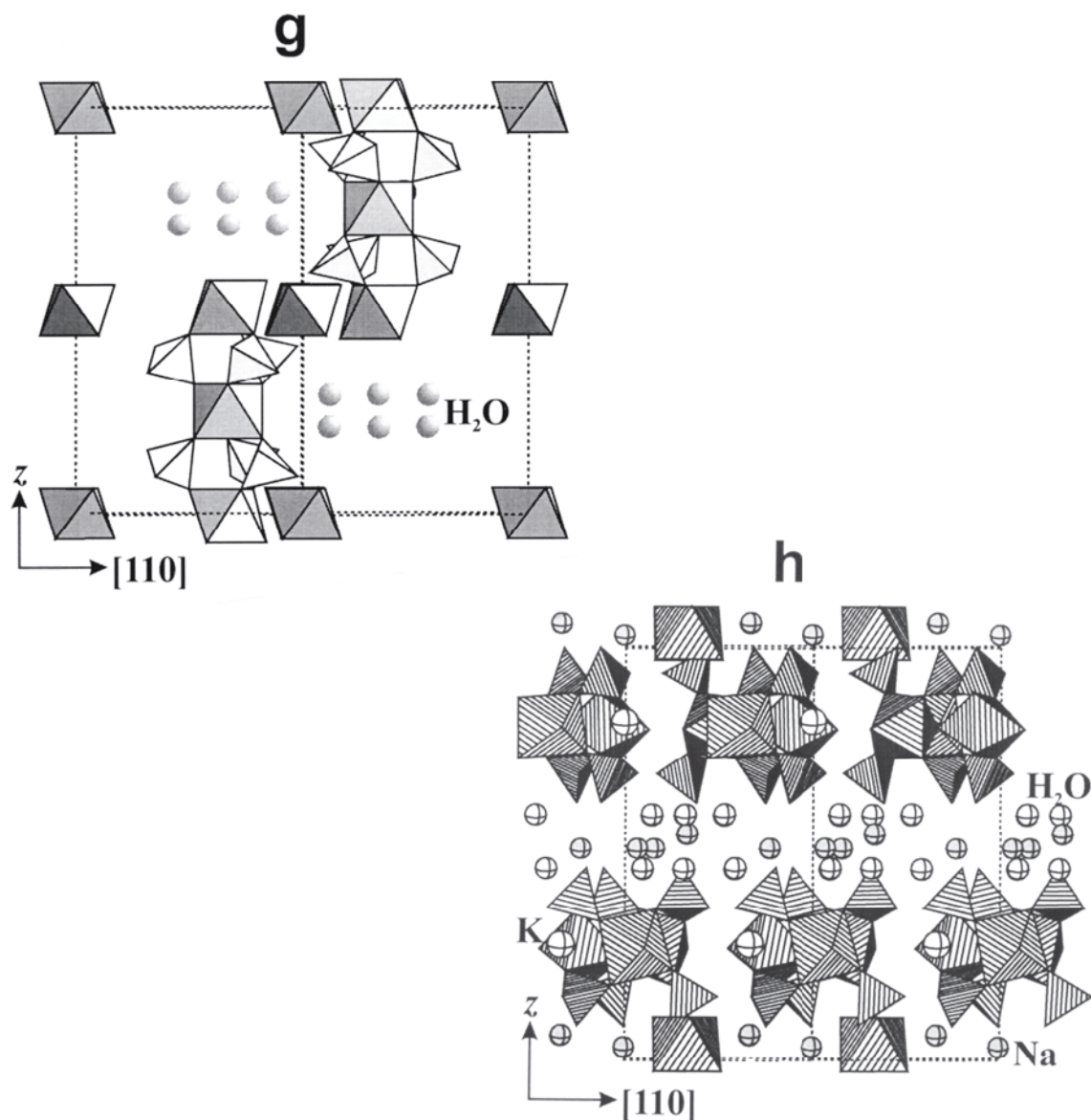
Figure 19, cont'd. (g) The structure of coquimbite, and (h) the structure of metavoltine.
