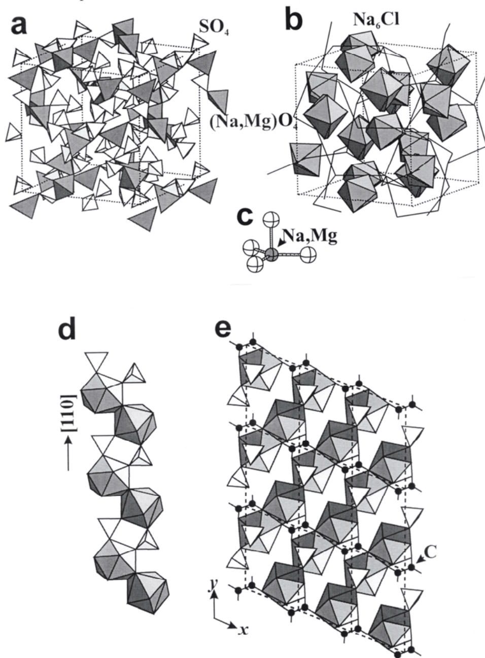
Figure 52. (a) The framework of [(\text{Na,Mg})\text{O}_4] trigonal pyramids and (\text{SO}_4) tetrahedra in d'ansite; (b) the positions of (\text{Na}_6\text{Cl}) octahedra in the framework of d'ansite, with the latter shown as a net; (c) coordination of the (\text{Na,Mg}) position in d'ansite; (d) the chain of (\text{REE})\text{O}_9 polyhedra and (\text{SO}_4) tetrahedra in coskrenite-(Ce); (e) the chains in coskrenite-(Ce) cross-linked by (\text{C}_2\text{O}_4) groups to form a sheet.
