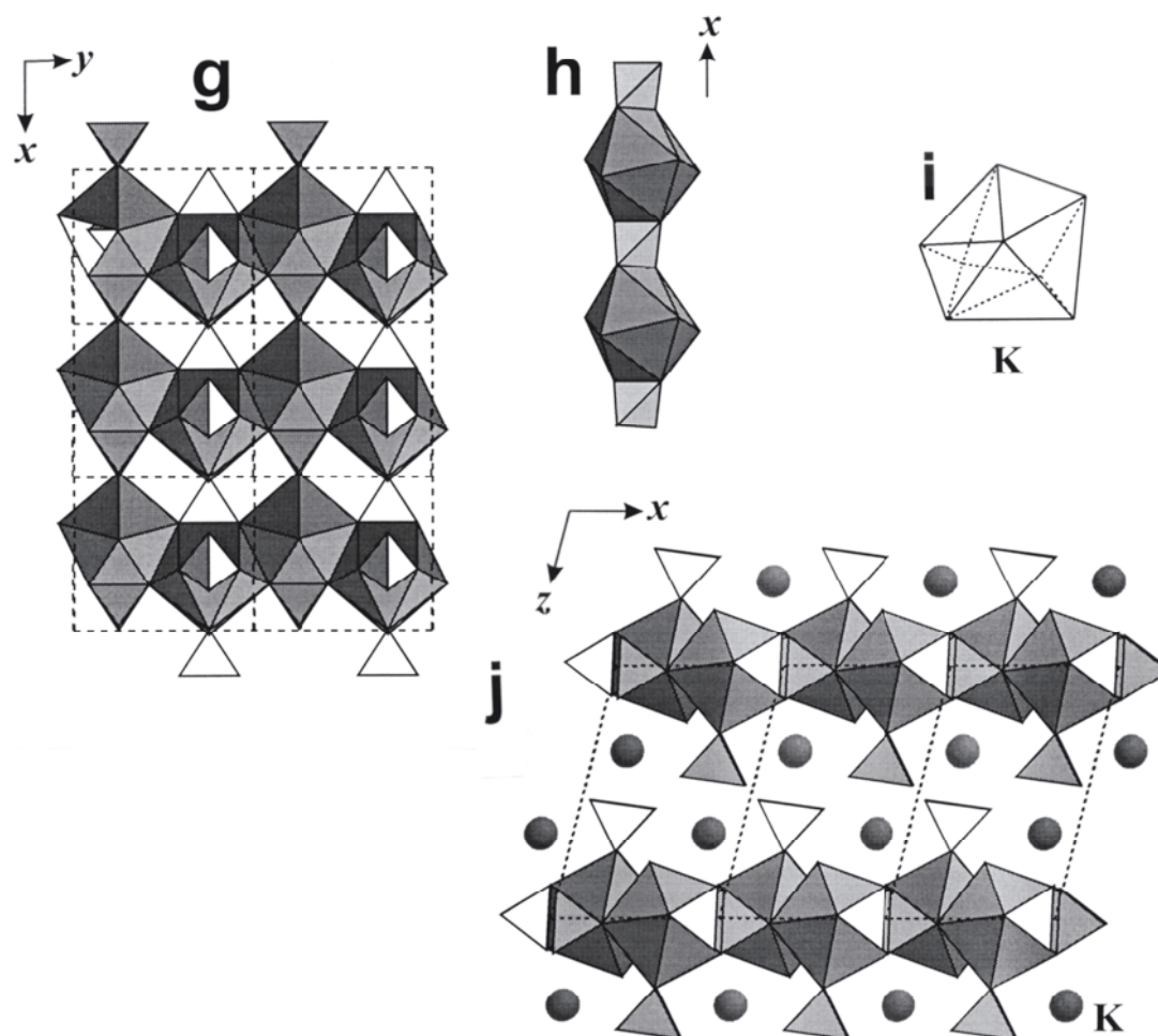
Figure 38, cont'd. (g) the structure of syngenite viewed along [001]; (h) the chain of edge-sharing (CaO 9 ) polyhedra and (SO 4 ) tetrahedra in syngenite; (i) the (K 8 ) 8 coordination polyhedron in syngenite; (j) the arrangement of layers of (CaO 9 ) polyhedra and (SO 4 ) tetrahedra with interstitial K in syngenite.
