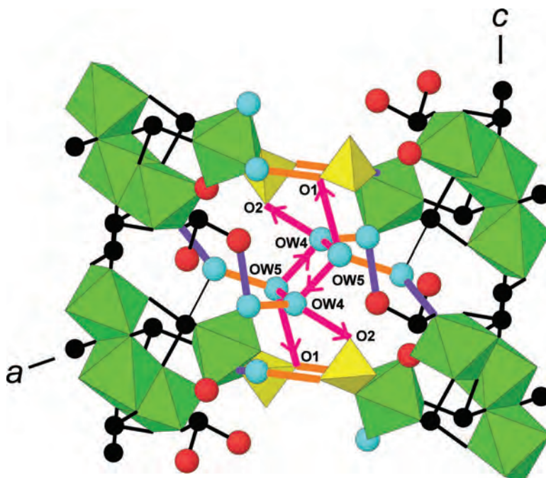
FIG. 14. The inter-slab hydrogen bonds (thick fuschia lines) donated by the interstitial {H 2 O} groups OW(4) and OW(5) in tamboite, projected down [010]. Legend as in Figure 13.
