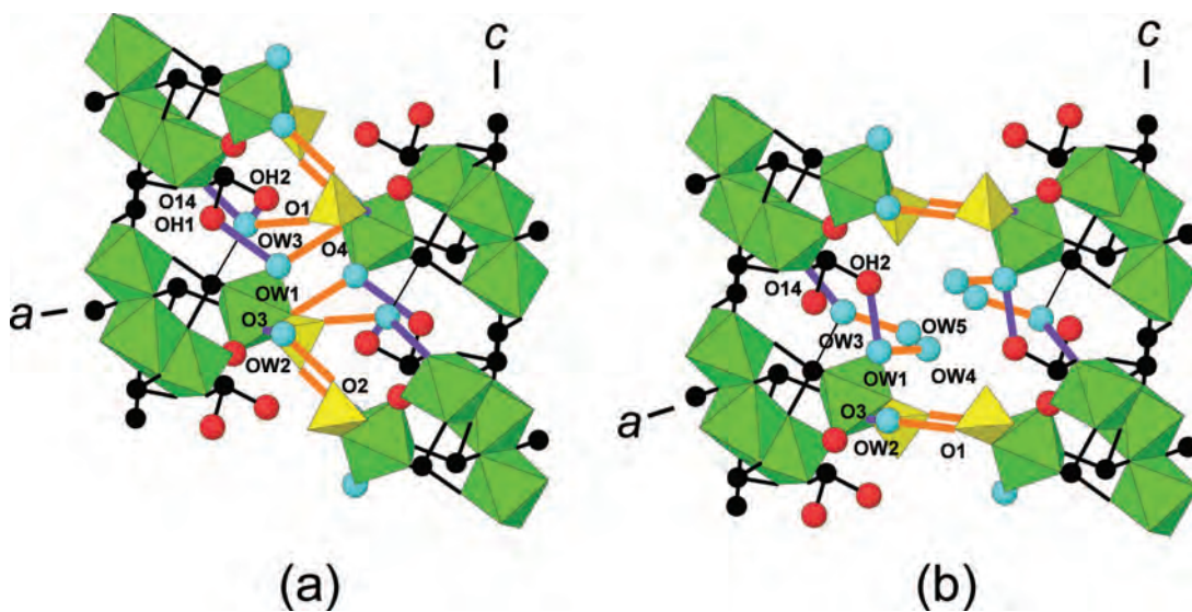
FIG. 13. The composite intra-slab hydrogen bonds (thick purple lines) and inter-slab hydrogen bonds (thick orange lines) involving the H 2 O groups bonded to cations in (a) metatamboite, (b) tamboite, projected down [010].
