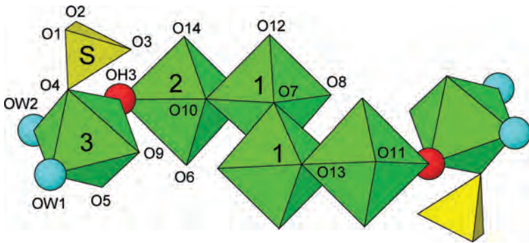
FIG. 7. The [\text{Fe}^{3+}_3(\text{SO}_4)\text{O}_{10}(\text{OH})(\text{H}_2\text{O})_2] ferric-sulfate-hydrate strand in metatamboite. Green polyhedra: \text{Fe}^{3+}\text{O}_6 octahedra; yellow polyhedra: \text{S}^{6+}\text{O}_4 tetrahedra; red circle: (OH) group; blue circle: ( \text{H}_2\text{O} ) group.
